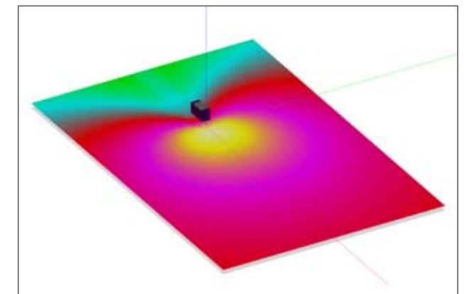
Vertical coverage in directional mode (100 hz)
