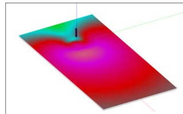
12 RS15 cluster over 75m/200ft, steered 15° down - Directional mode
