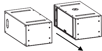
"FACE TO FACE" CONFIGURATION
