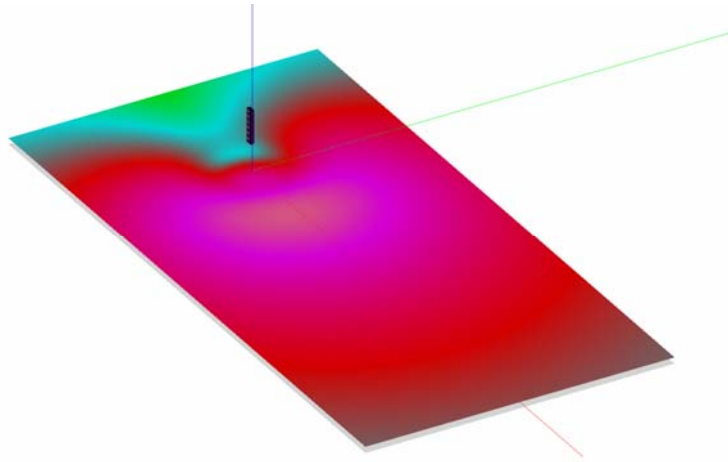
12 RS15 “ALTERNATE” CLUSTER OVER 75M/200FT, STEERED 15° DOWN
