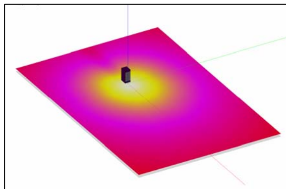
VERTICAL COVERAGE IN OMNI MODE (100 HZ)
