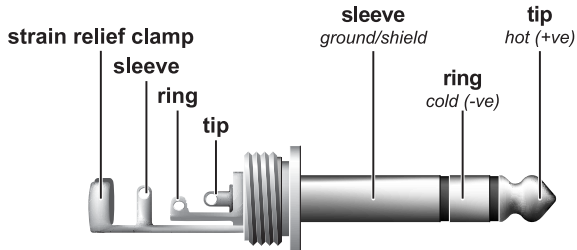
Fig. 8.3: 1/4" TRS connector
