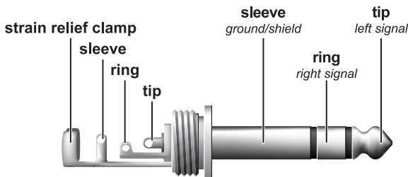
Fig. 8.4: Stereo headphones connector
