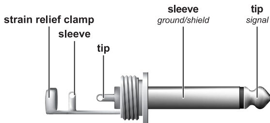
Fig. 8.2: 1/4" TS connector
