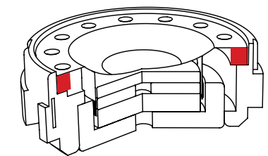
> Cross-section of the TNF tweeter. Poron's physical properties provide improved control over the mobile assembly in the magnetic parts.
