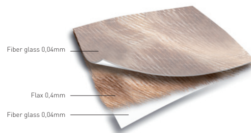
> Flax sandwich Details for midrange driver
