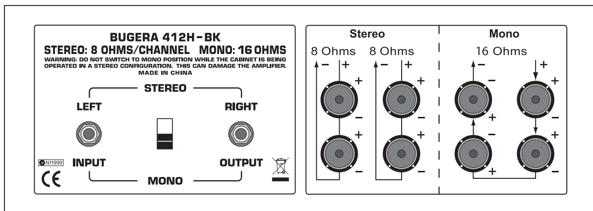
Rear panel
