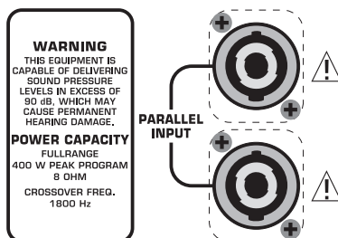
Fig. 1.1: B1520 PRO connector panel (B2520PRO/B1220 PRO's are similar)
