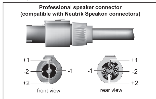
Fig. 1.3: Speakon connector
