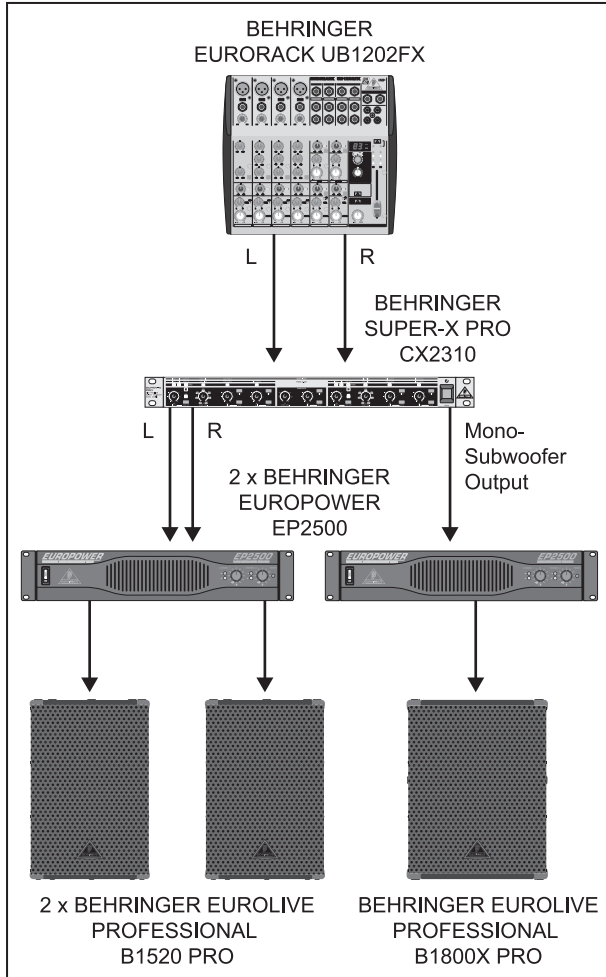
Fig. 6.2: Stereo operation with a subwoofer
